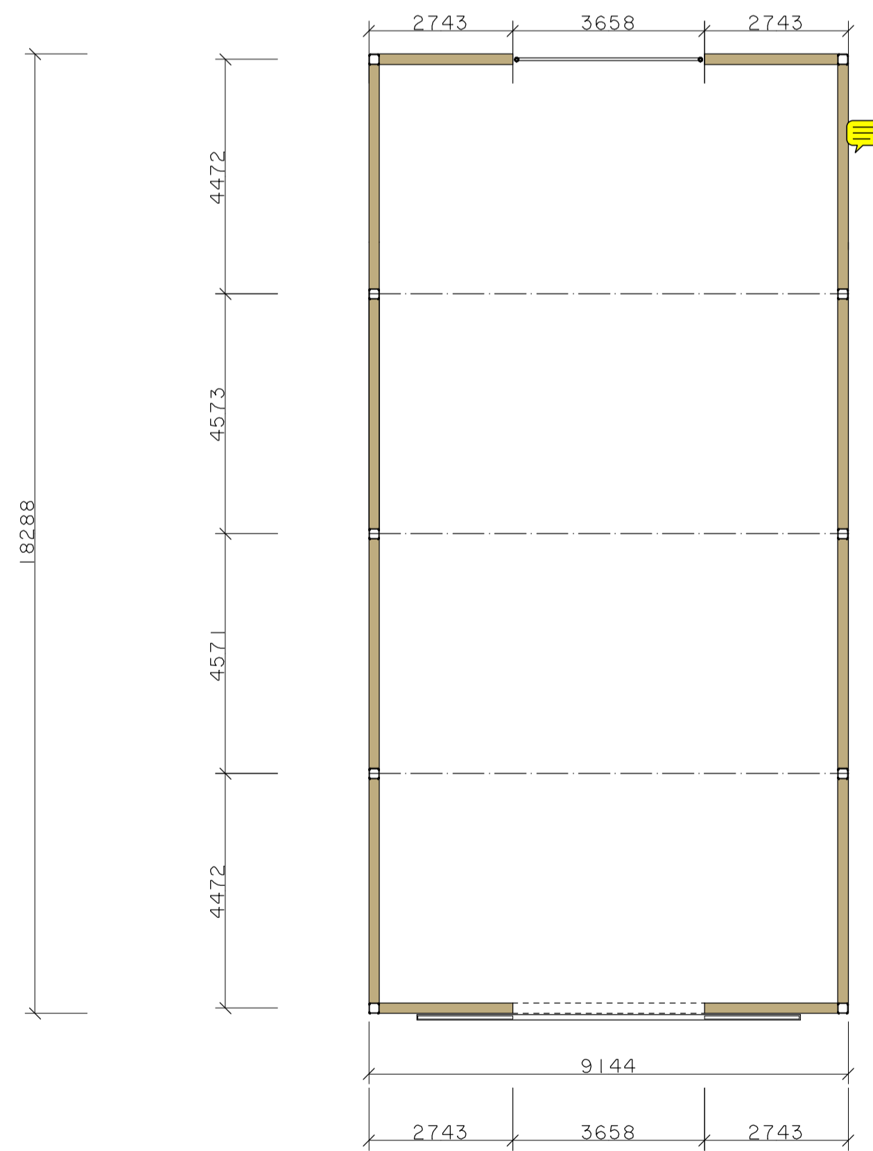
FLOOR LAYOUT PLAN
