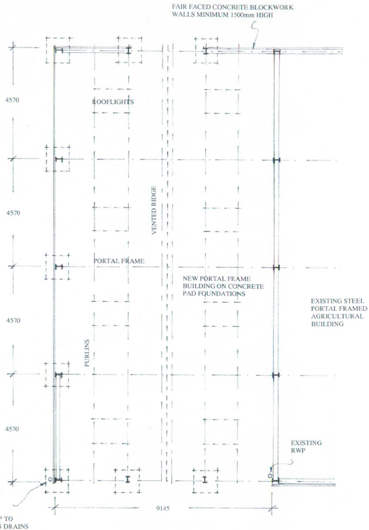
LAYOUT PLAN
