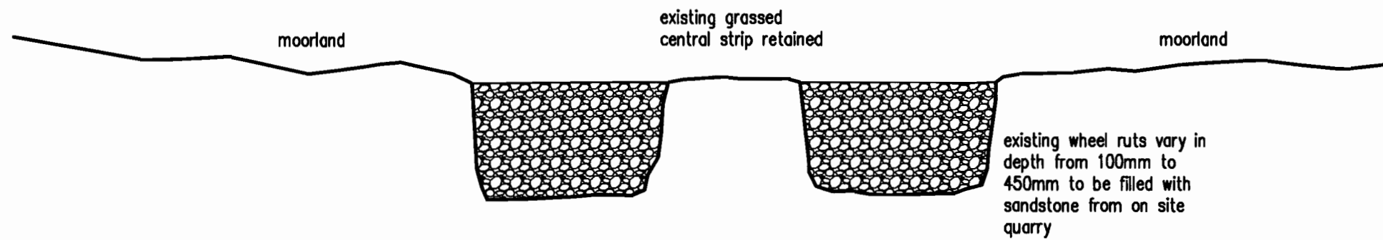
Cross Section Thro' Road from Point A - B
