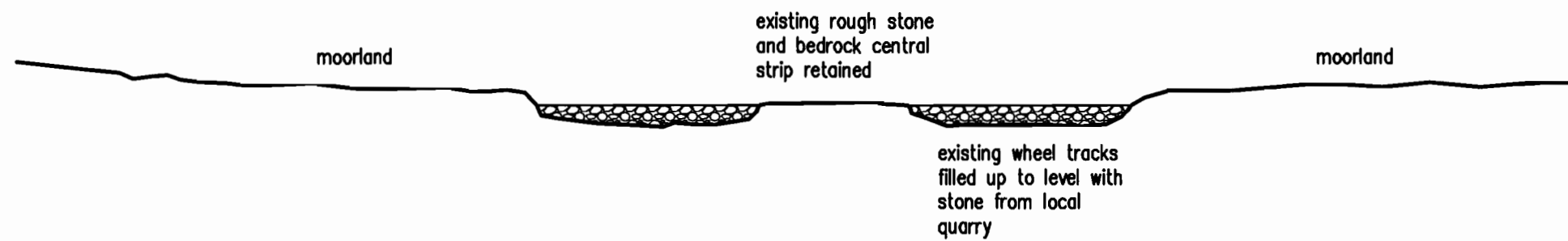
Cross Section Thro' Road from Point C - D
